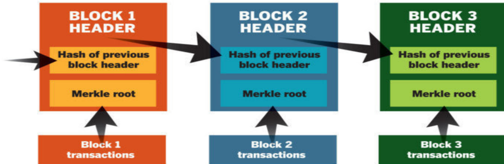
SIMPLIFIED BITCOIN BLOCK CHAIN
